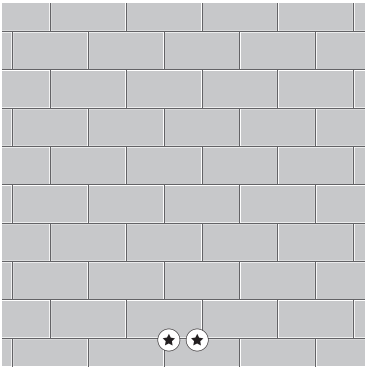
Half cut tiles in brickwork, with inlay strip 砖制半切块材，带嵌条
